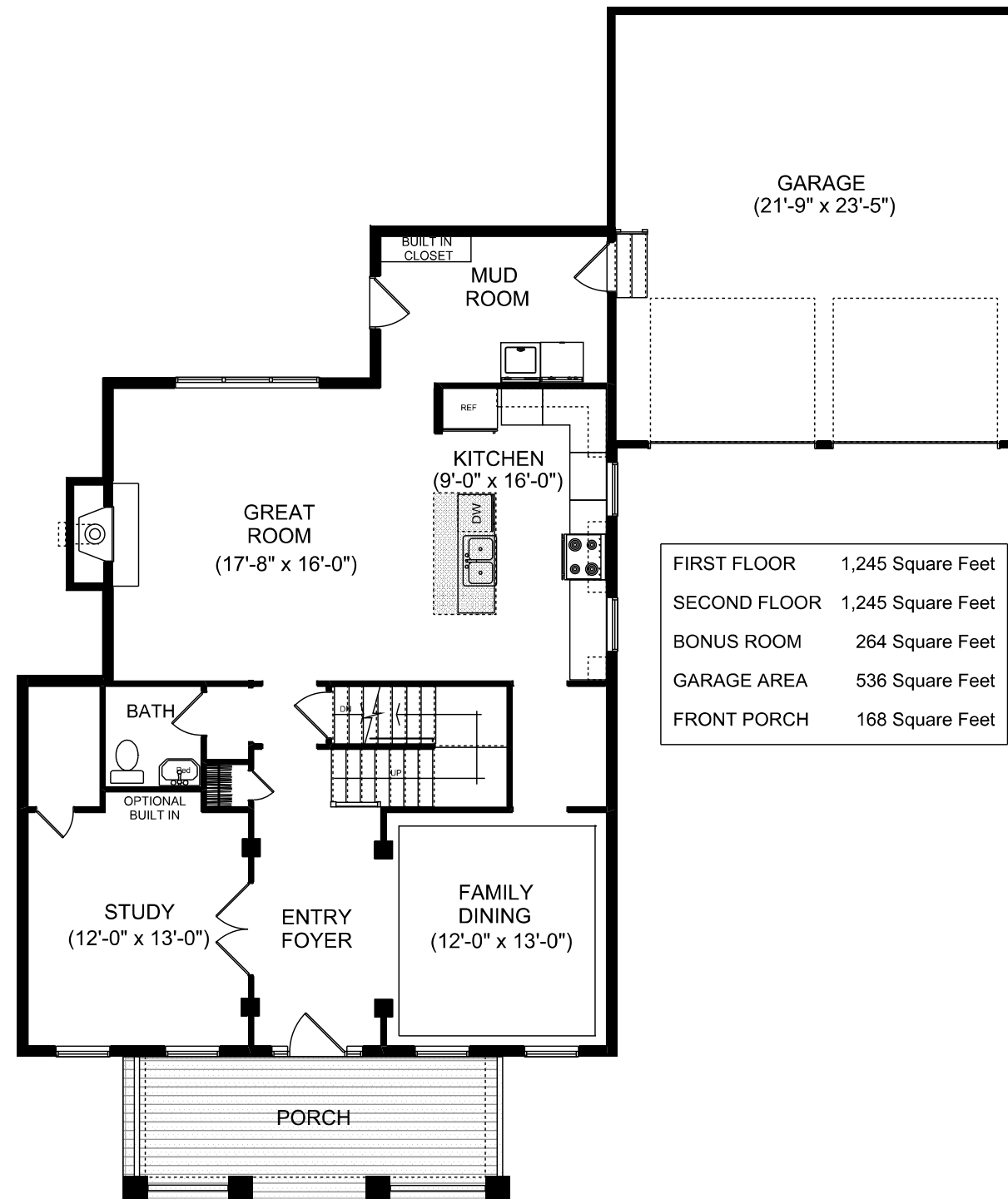
Lenox Standard First Floor Plan
