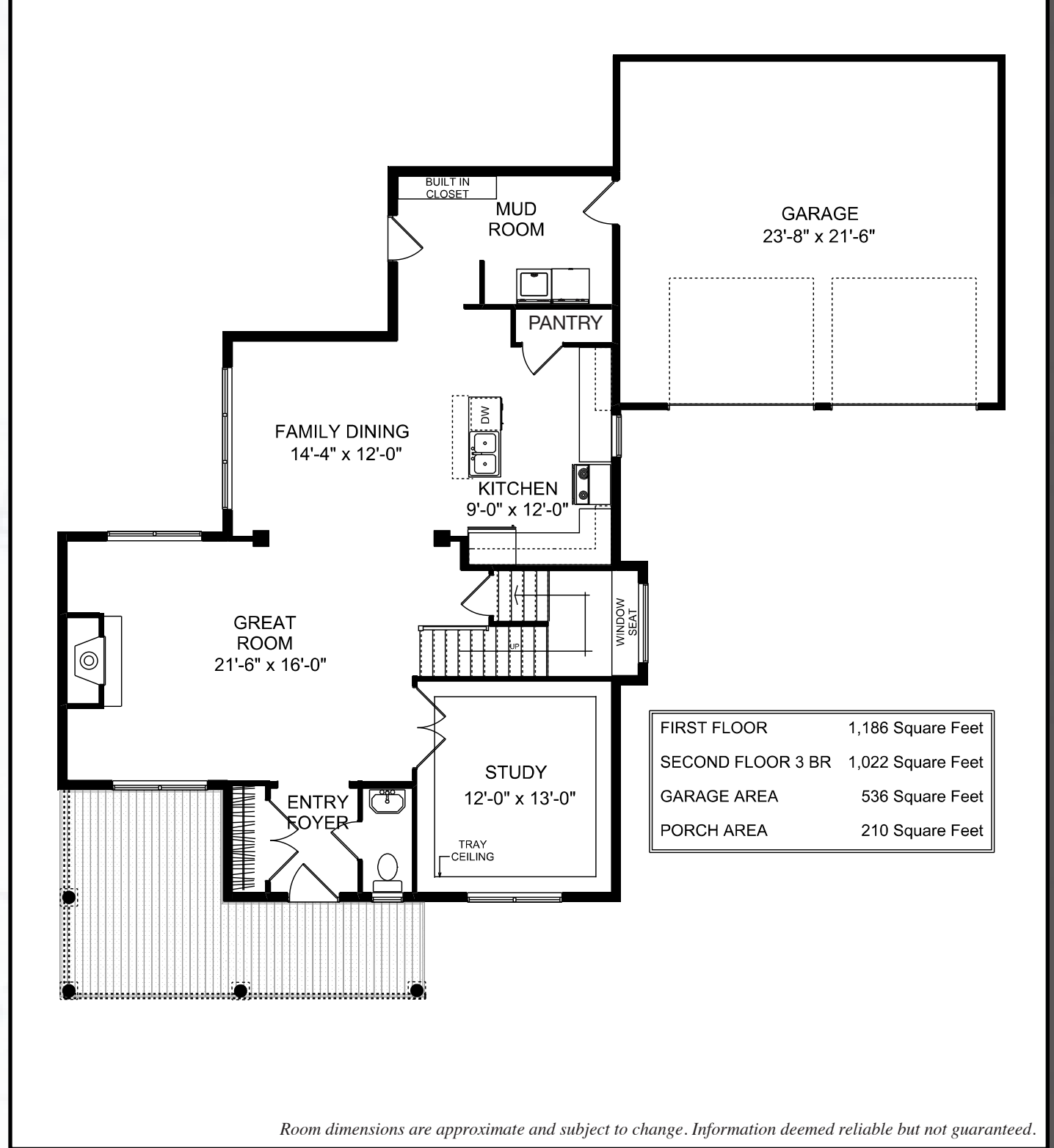
Wendell Standard First Floor Plan
